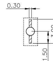
DETAIL D(4:1)
